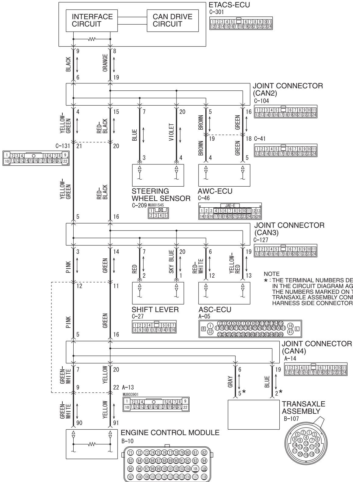
CAN-C Communication Circuit <TC-SST>
