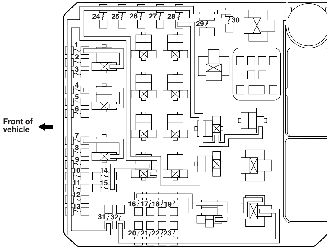
Relay box in engine compartment
